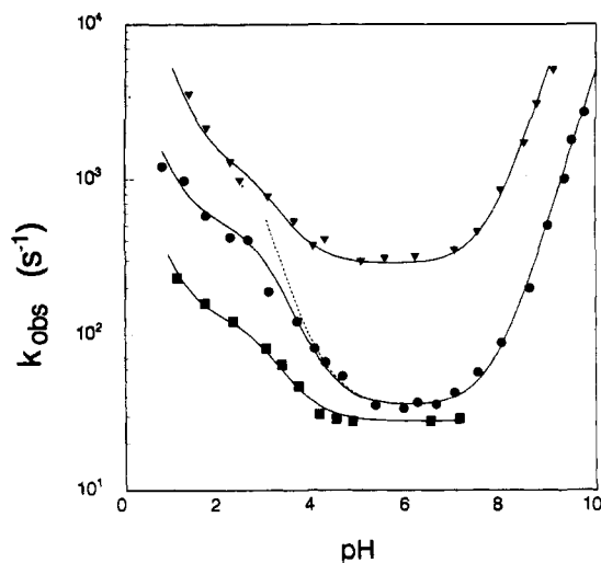
Figure 2. Measured rates of breakdown into flavin and hydrogen peroxide of three flavin 4a-OOH species in water as a function of the pH. ▼, FIH-4a-OOH; ●, 3MeTARFH-4a-OOH; ■ 5TARF-4a-OOH.
